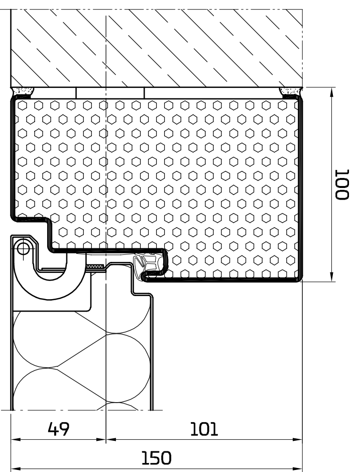
Block 100 00 / 30
