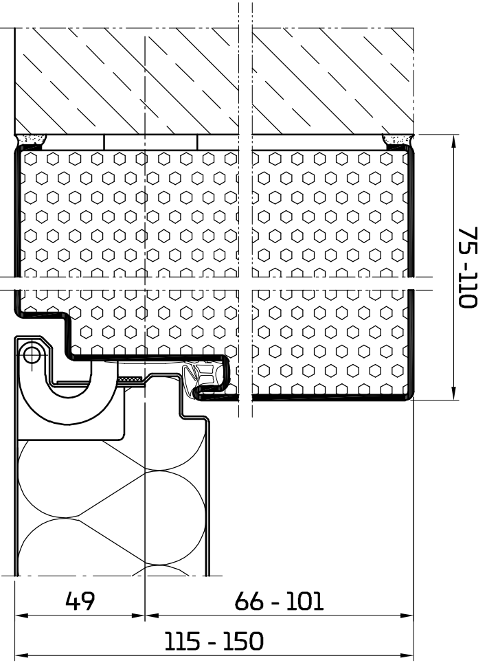
Block Variabel 00 / 30
