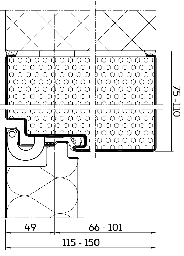
Block Variabel 00 / 30
