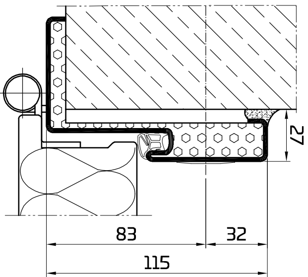
Eckzarge 27
