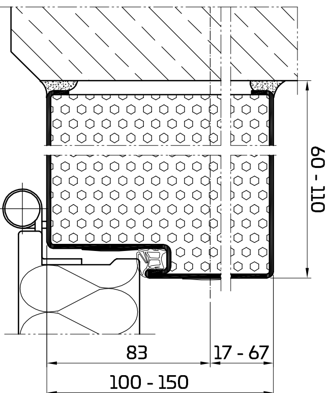
Blockzarge 70 / 100
