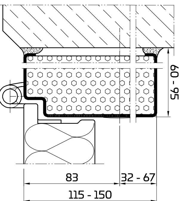
Blockzarge 60 / 85
