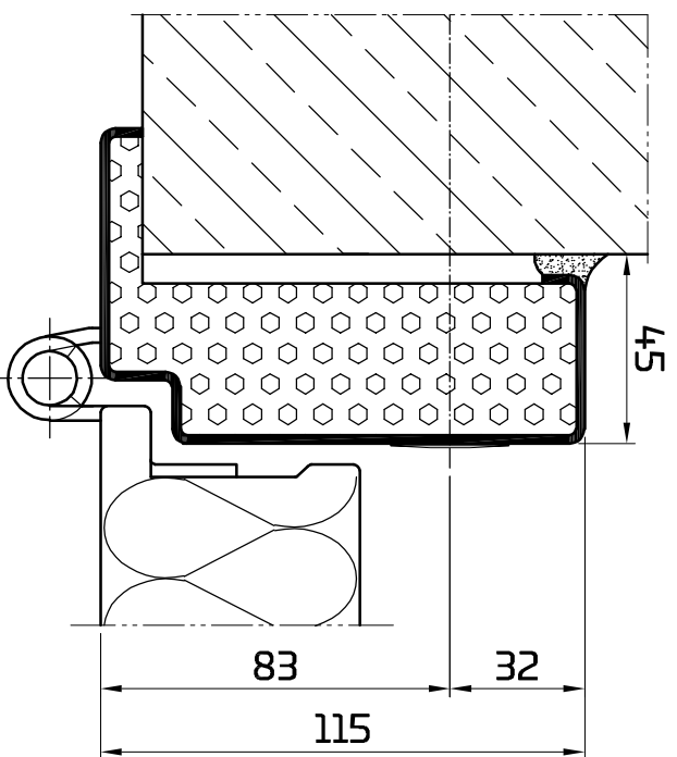
Eckzarge 45
