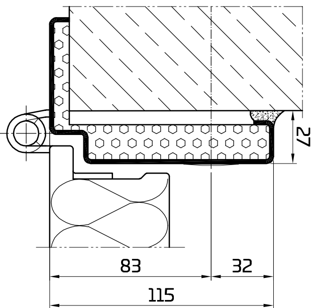
Eckzarge 27
